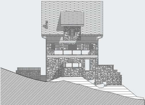
EAST ELEVATION
